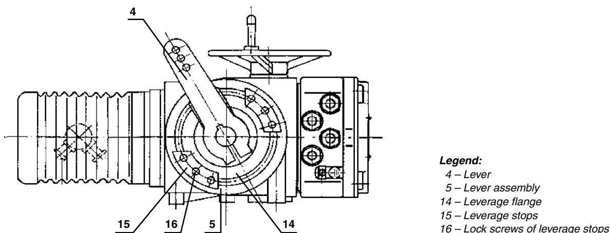
Fig. 4 - Level system
